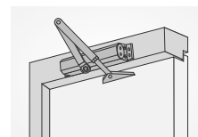
Door Frame Installation
